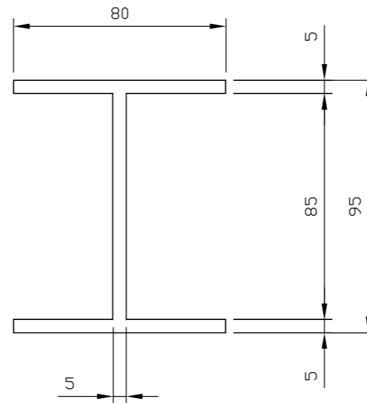
STD JOINING SECTION L-121019-RAW-DT-07
