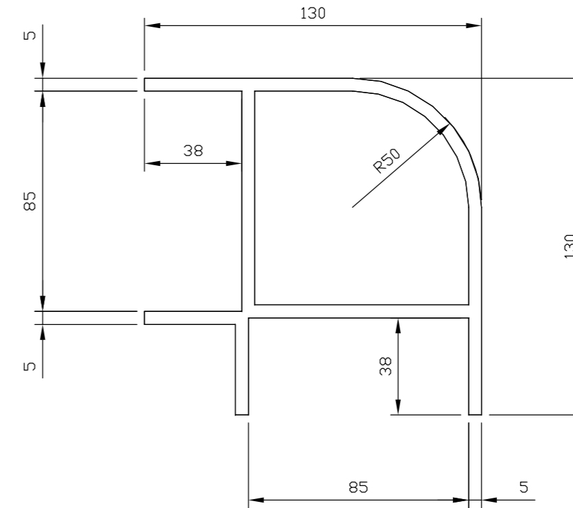
STD 90° CORNER L-121019-RAW-DT-06
